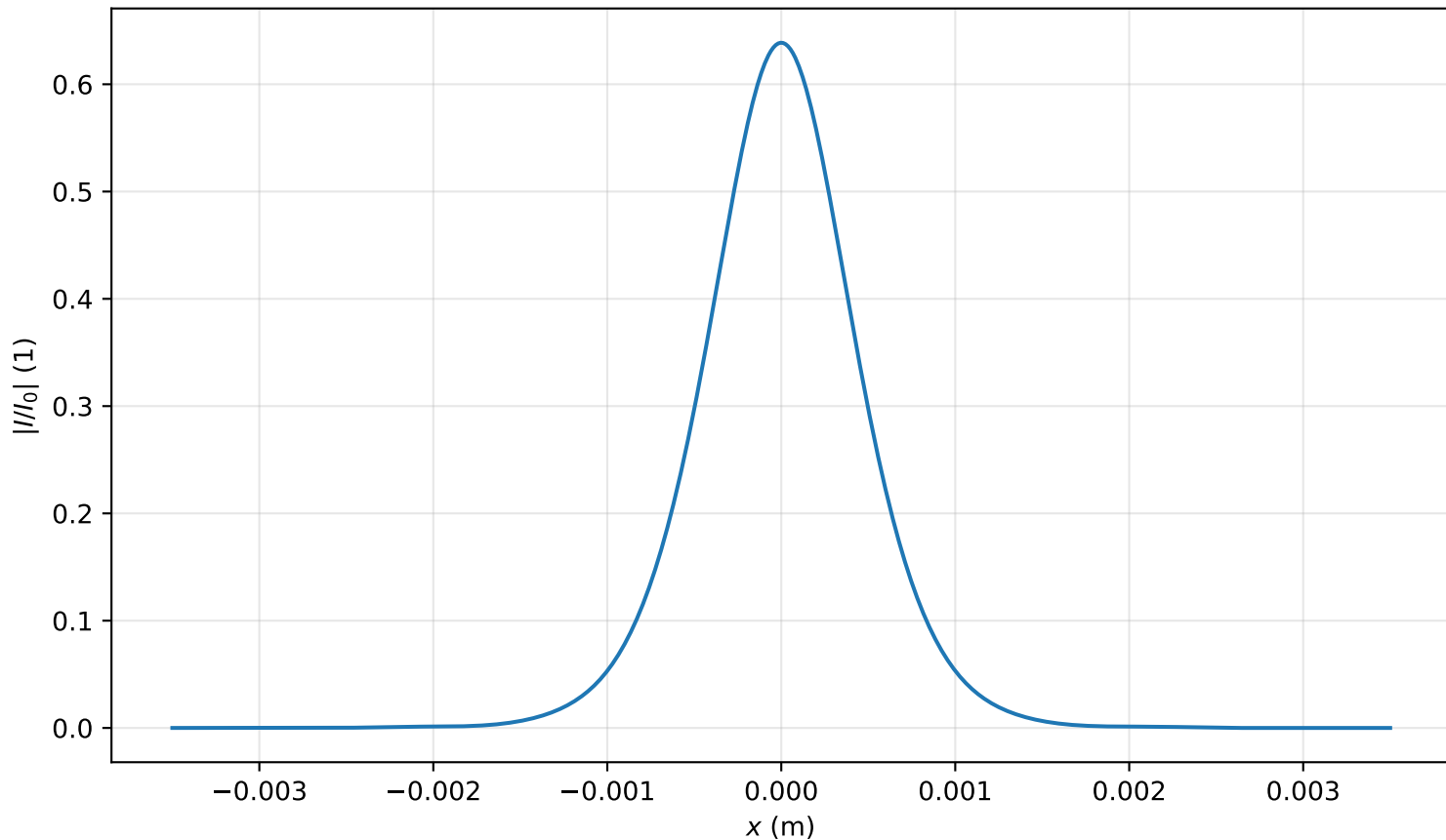
Intensity profile I(x, y = 0, z = 3.901m)/I_0 , P_{in}=0.7P_{cr} , artificial time
